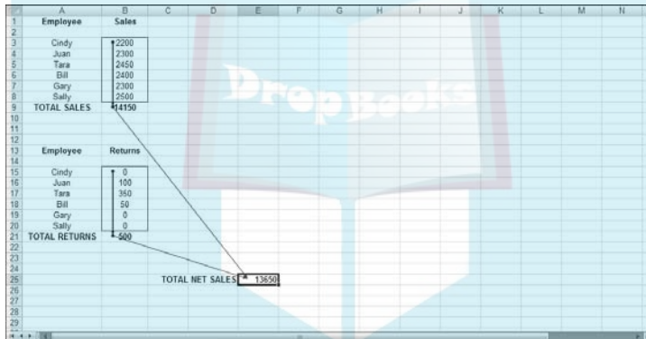
Figure 4-14: Tracing formulas.
